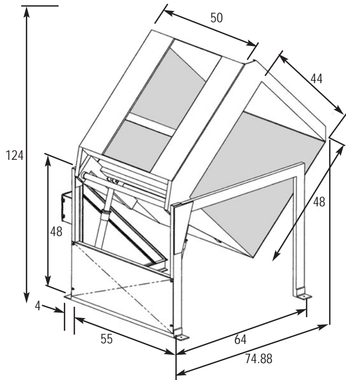
Box dumper, side load
