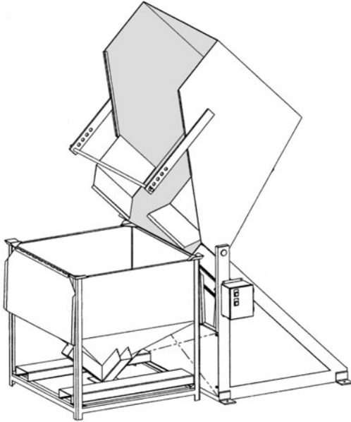
Box dumper with enclosed funnel
