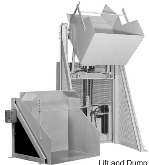
Rear Load Box Dumper
