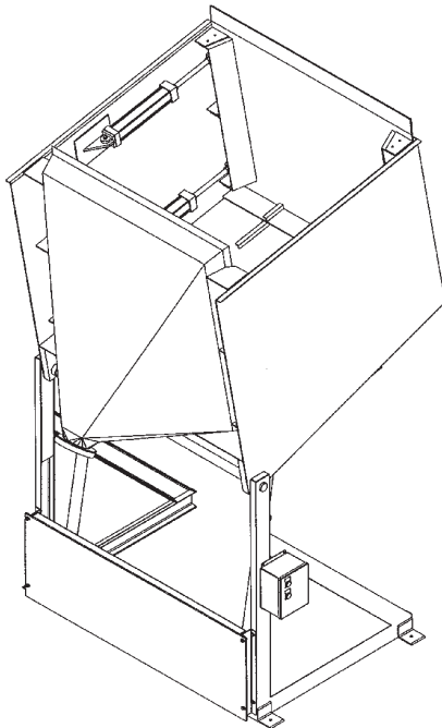
Lift and seal box dump
